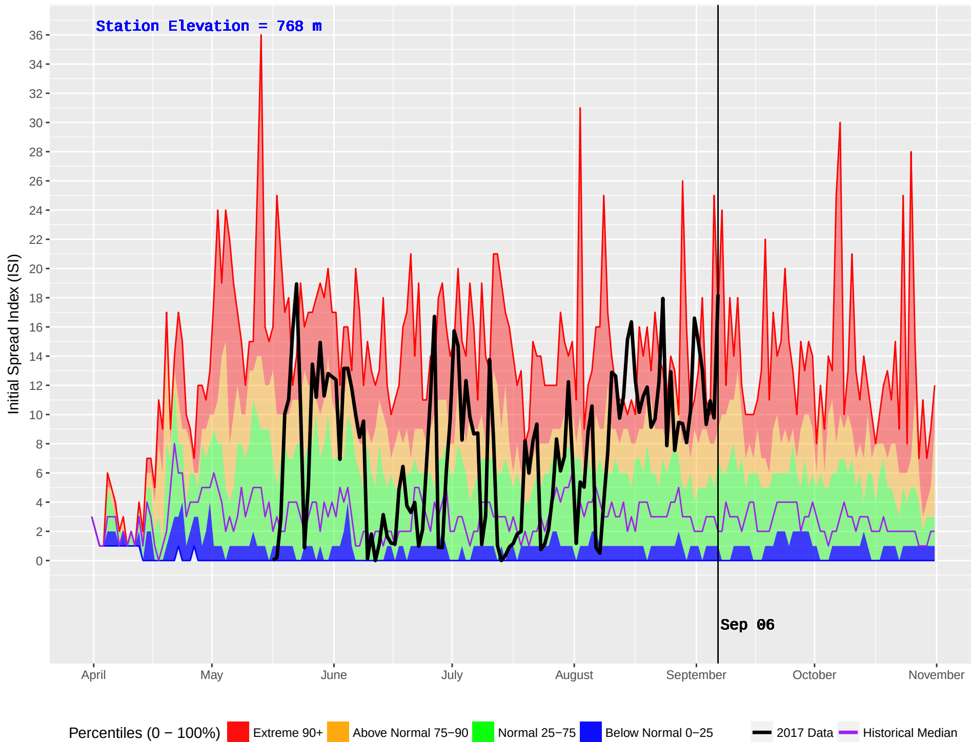
GRAHAM (124) : Historical (1979–2016) and Current (2017) Noon Initial Spread Index (ISI)
