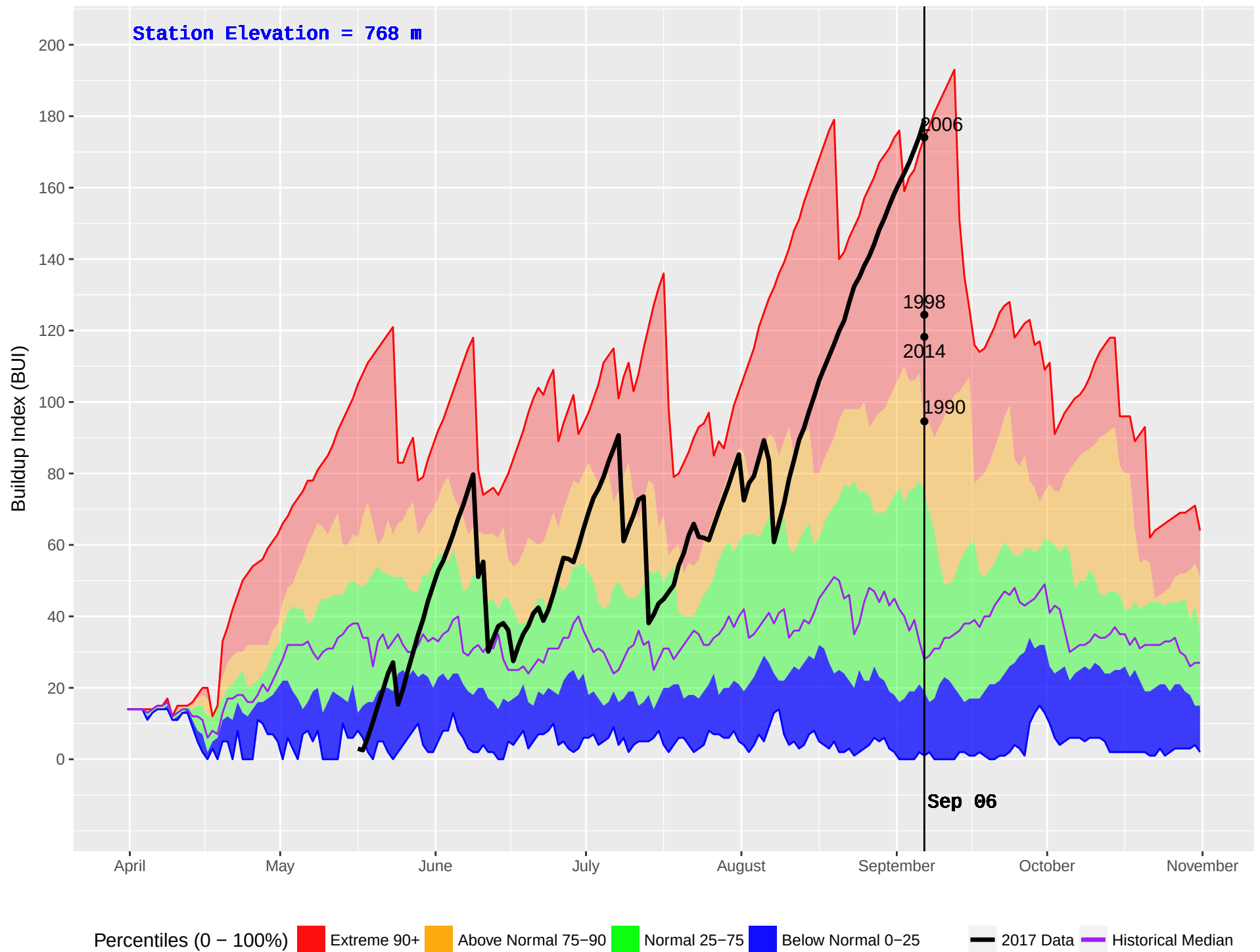
GRAHAM (124) : Historical (1979–2016) and Current (2017) Noon Buildup Index (BUI)
