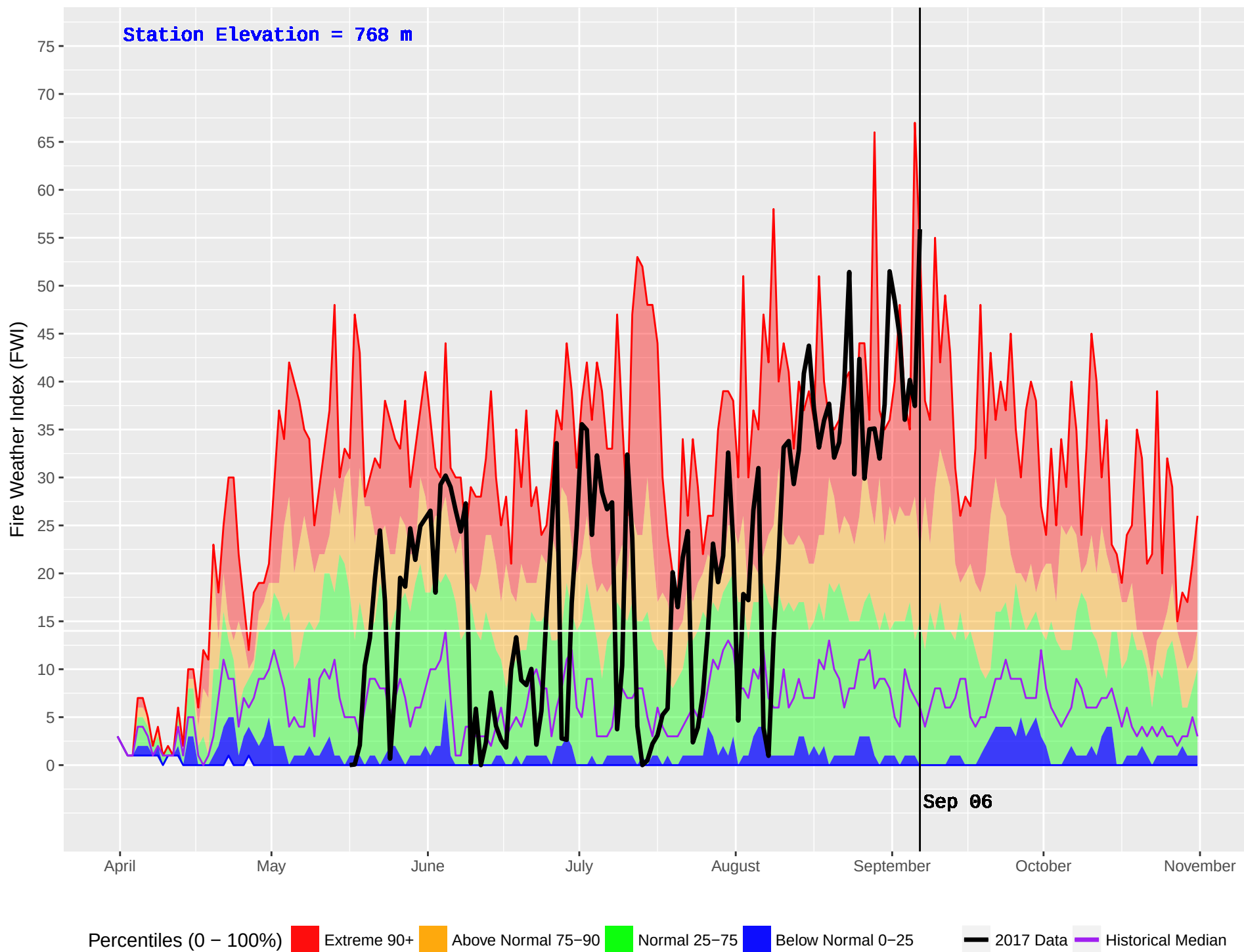
GRAHAM (124) : Historical (1979–2016) and Current (2017) Noon Fire Weather Index (FWI)
