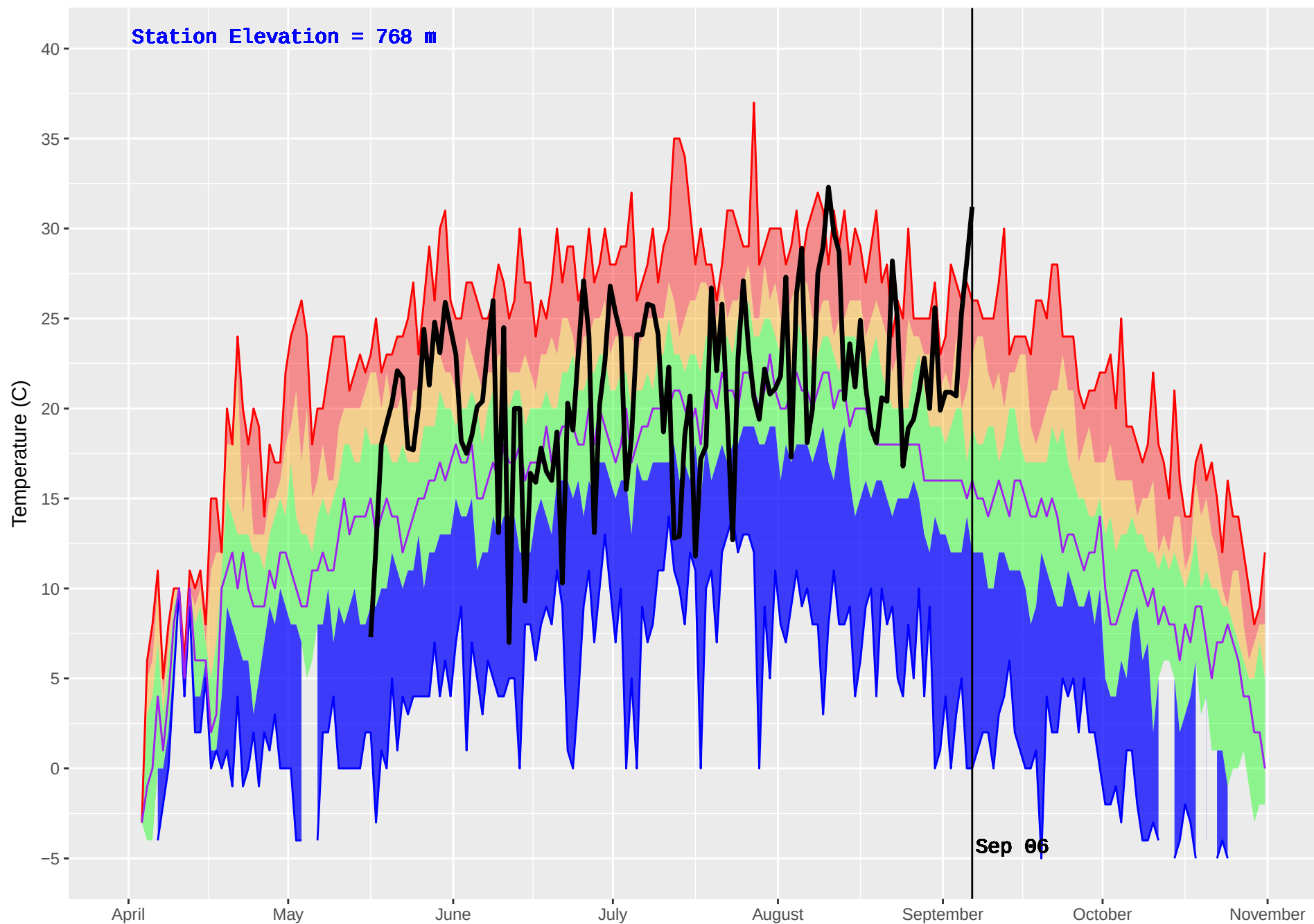
GRAHAM (124) : Historical (1979–2016) and Current (2017) Noon Temperature
