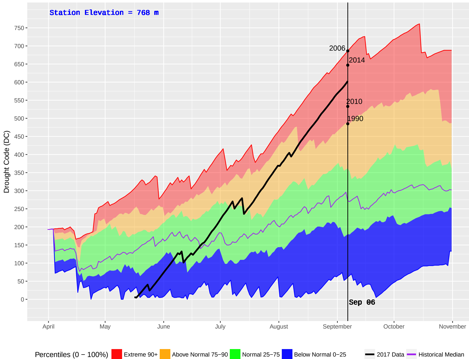
GRAHAM (124) : Historical (1979–2016) and Current (2017) Noon Drought Code (DC)
